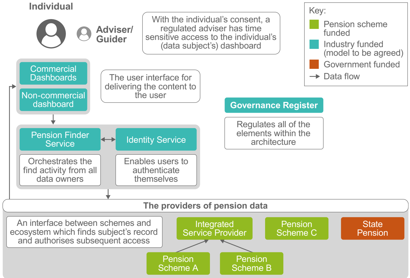
Diagram 1: Model of a dashboard ecosystem
